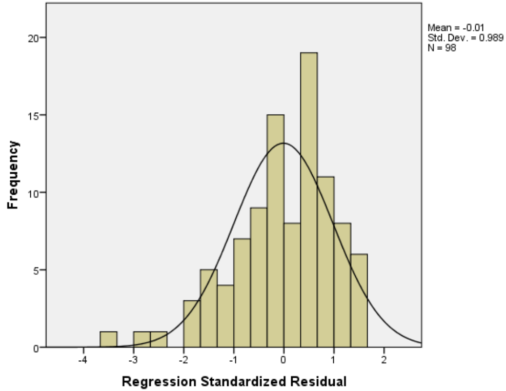
Figure 4-2. Histogram: Dependent Variable Work Ability Index Scores Standardized Residuals.
